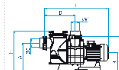
COLORADO pump with strainer Bomba COLORADO con pre-filtro
